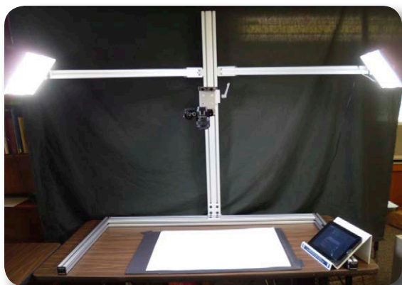
Figure 4: The final Preservation Capture System design constructed of aluminum, in use at the PCS Pilot Project headquarters.
